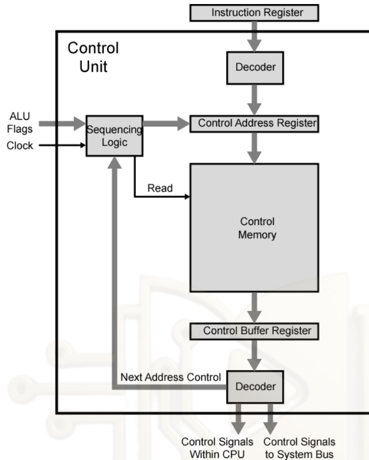
Fig: Functioning of Micro programmed Control Unit
